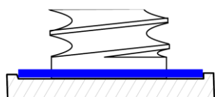
stepped bearing according to DIN 3852 E
